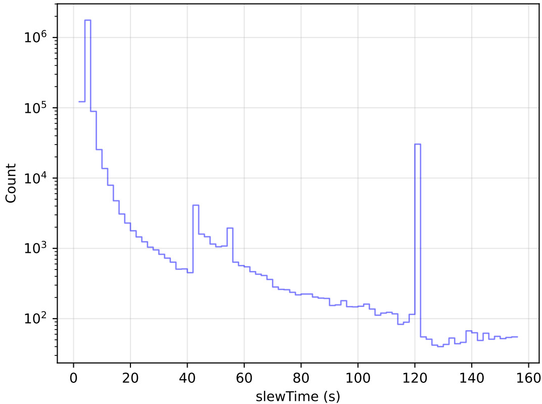
internal_u_expt45_nscale1.0v3.4_10yrs All visits: Slew Time Histogram
