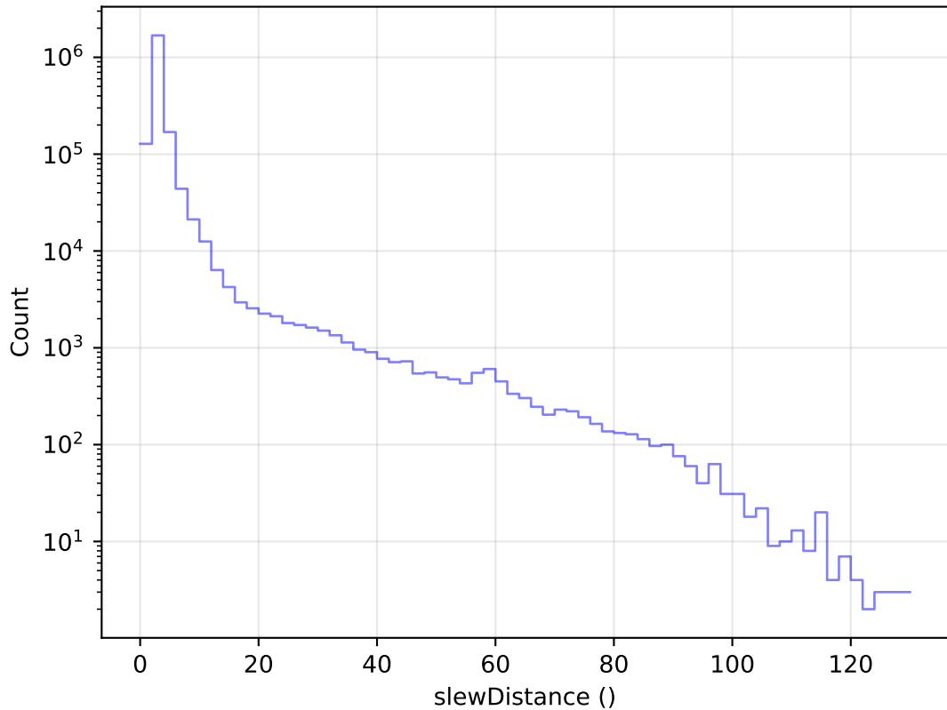
internal_u_expt45_nscale1.0v3.4_10yrs All visits: Slew Distance Histogram
