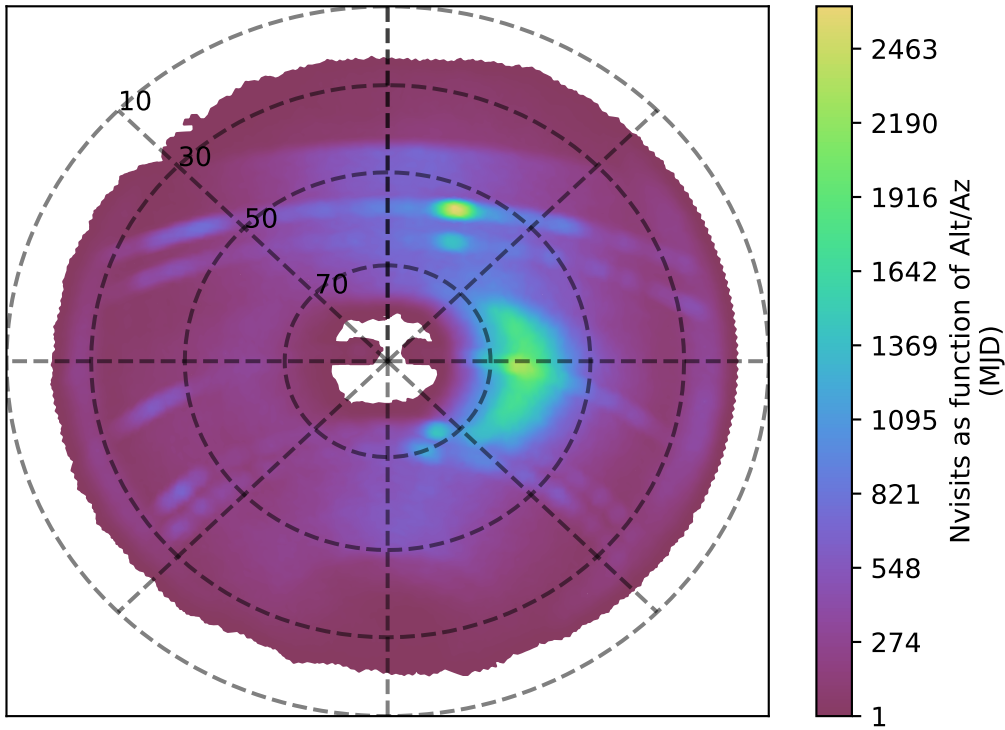
internal_u_expt45_nscale1.0v3.4_10yrs z band: Nvisits as function of Alt/Az
