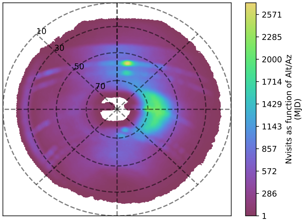
internal_u_expt45_nscale1.0v3.4_10yrs r band: Nvisits as function of Alt/Az
