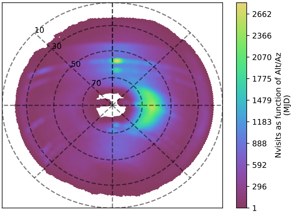
internal_u_expt45_nscale1.0v3.4_10yrs i band: Nvisits as function of Alt/Az
