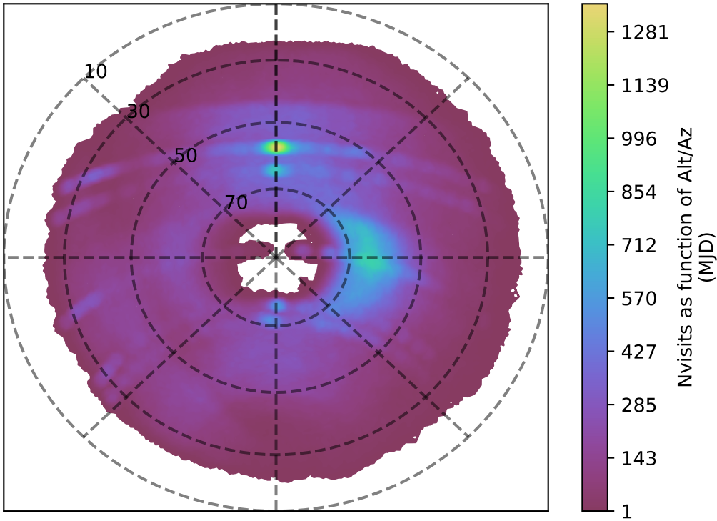
internal_u_expt45_nscale1.0v3.4_10yrs g band: Nvisits as function of Alt/Az
