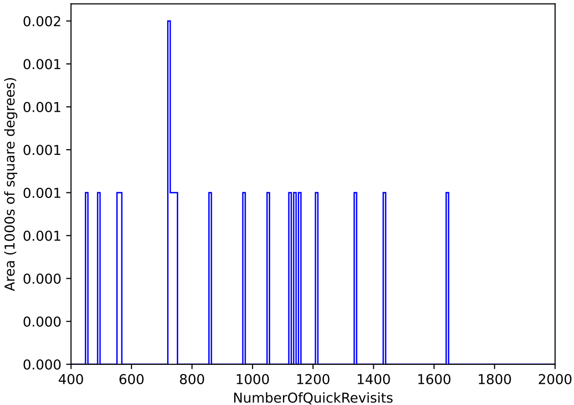
internal_u_expt45_nscale1.0v3.4_10yrs WFD: NumberOfQuickRevisits
