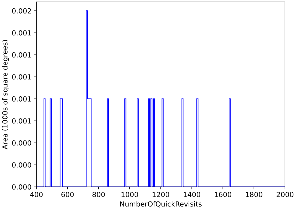
internal_u_expt45_nscale1.0v3.4_10yrs All sky: NumberOfQuickRevisits
