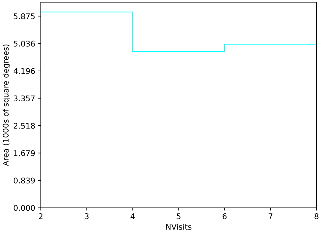
internal_u_expt45_nscale1.0v3.4_10yrs Yr 3-4 u band: NVisits
