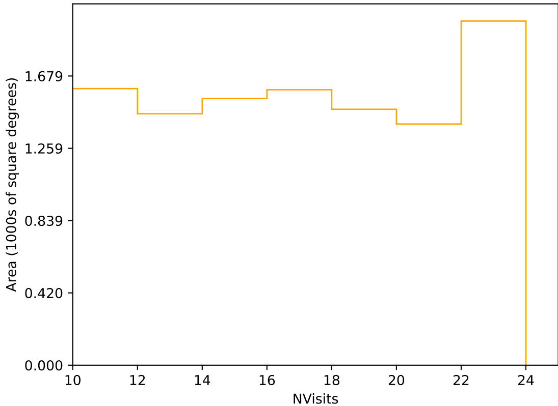
internal_u_expt45_nscale1.0v3.4_10yrs Yr 3-4 r band: NVisits
