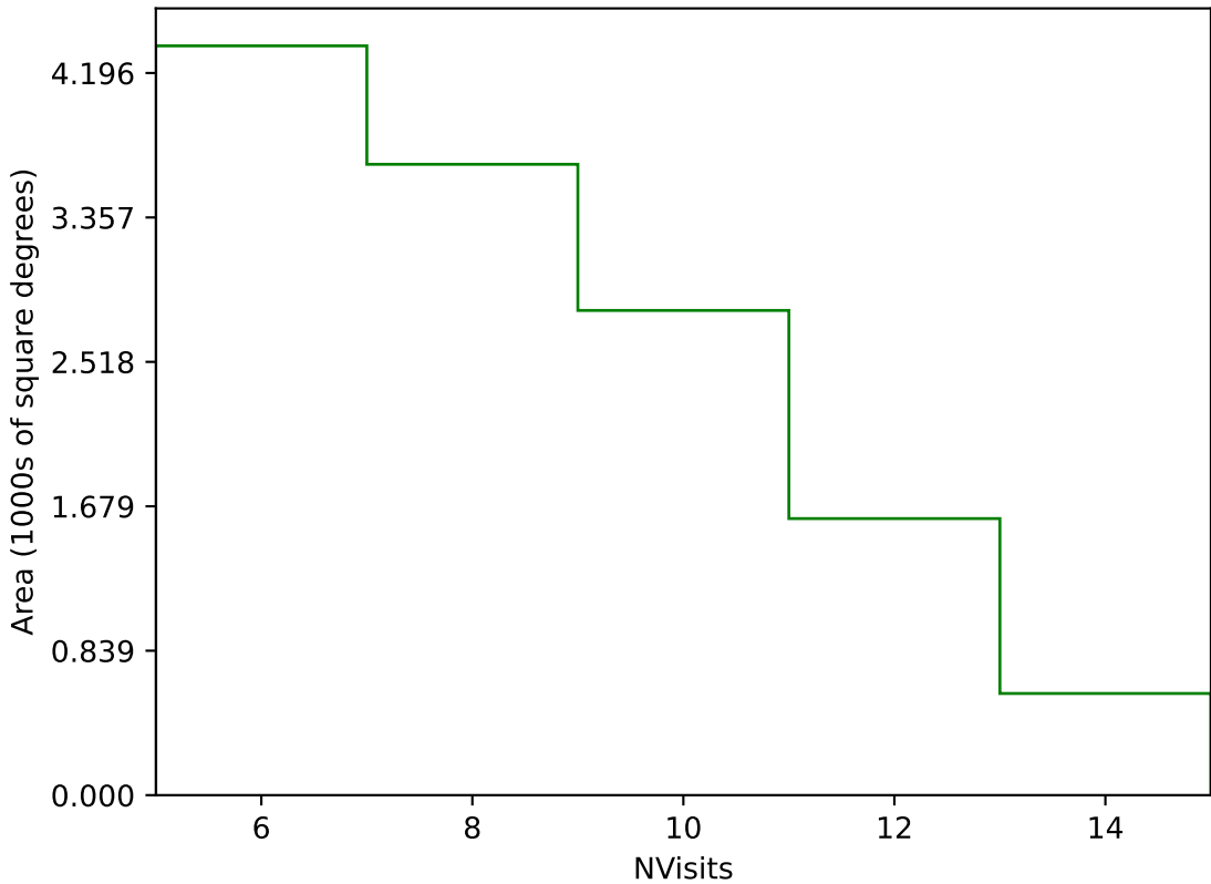
internal_u_expt45_nscale1.0v3.4_10yrs Yr 3-4 g band: NVisits
