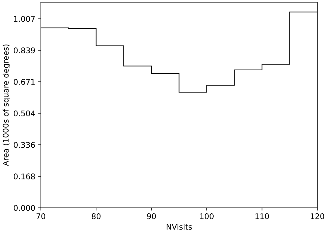
internal_u_expt45_nscale1.0v3.4_10yrs Yr 3-4 all bands: NVisits
