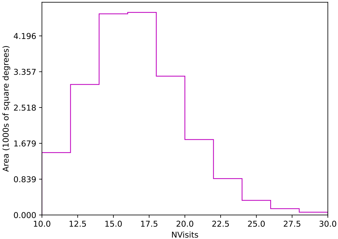
internal_u_expt45_nscale1.0v3.4_10yrs Yr 1 z band: NVisits
