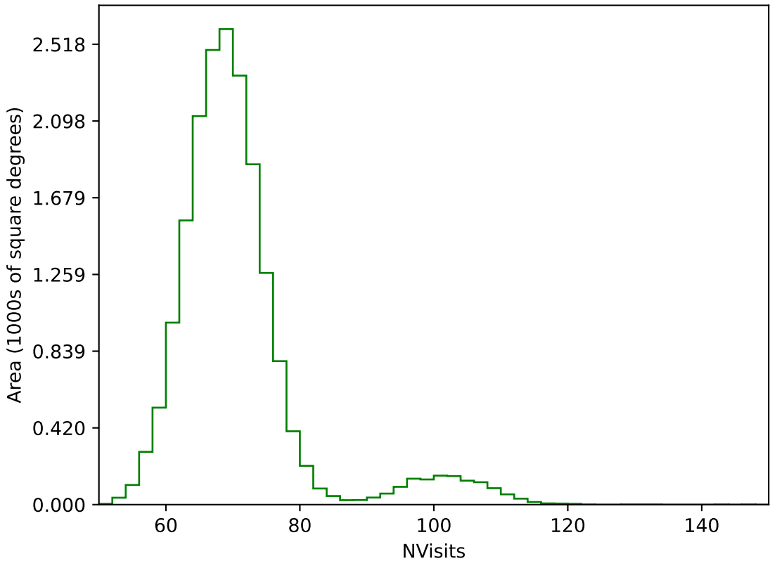
internal_u_expt45_nscale1.0v3.4_10yrs WFD g band: NVisits
