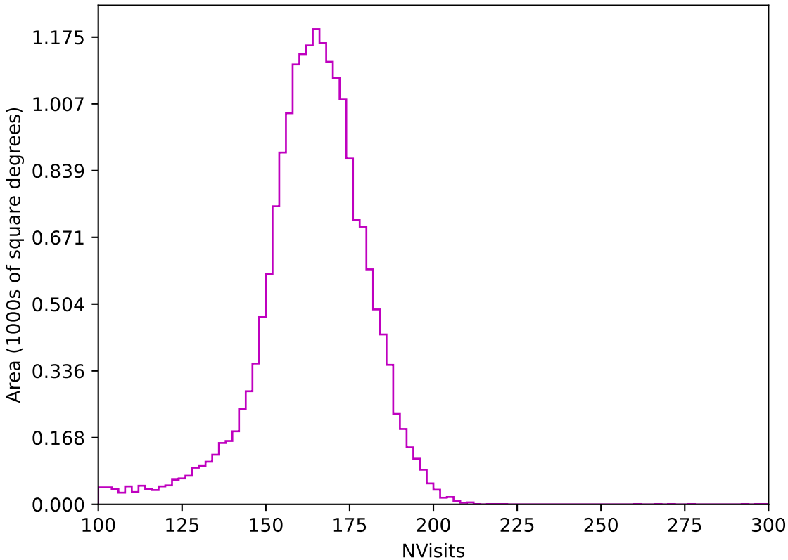
internal_u_expt45_nscale1.0v3.4_10yrs All sky z band: NVisits
