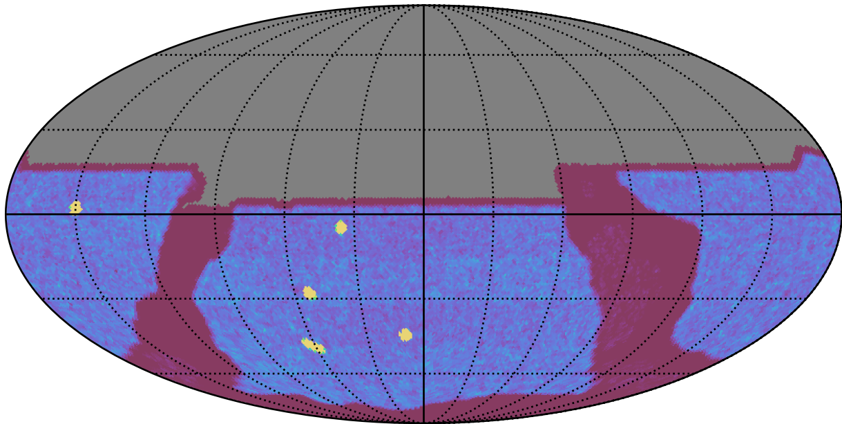
internal_u_expt45_nscale1.0v3.4_10yrs All sky y band: NVisits
