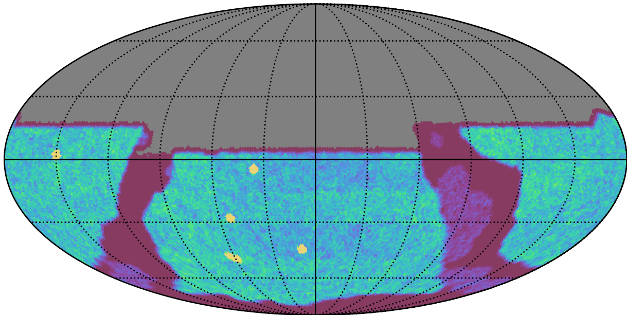
internal_u_expt45_nscale1.0v3.4_10yrs All sky u band: NVisits
