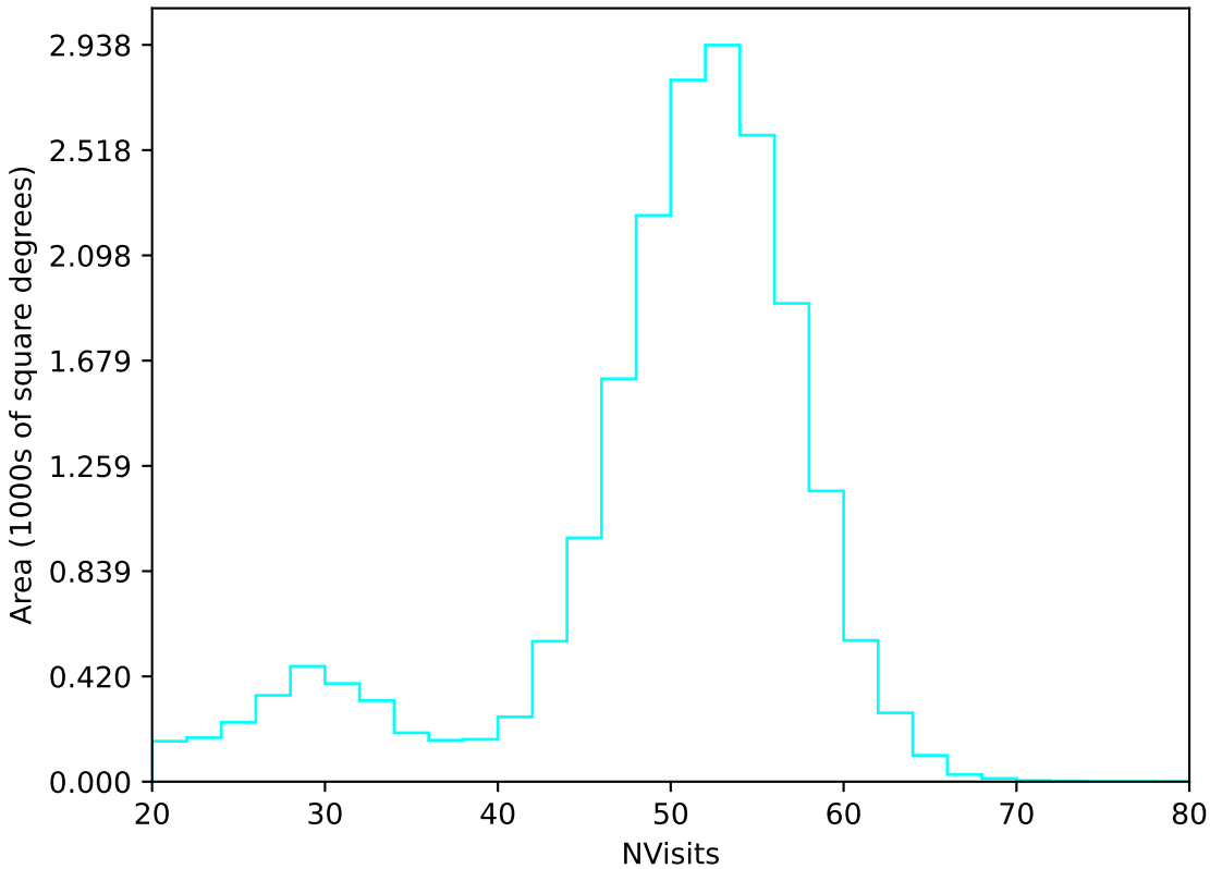
internal_u_expt45_nscale1.0v3.4_10yrs All sky u band: NVisits
