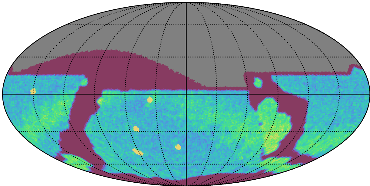
internal_u_expt45_nscale1.0v3.4_10yrs All sky r band: NVisits
