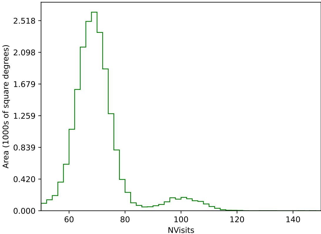
internal_u_expt45_nscale1.0v3.4_10yrs All sky g band: NVisits
