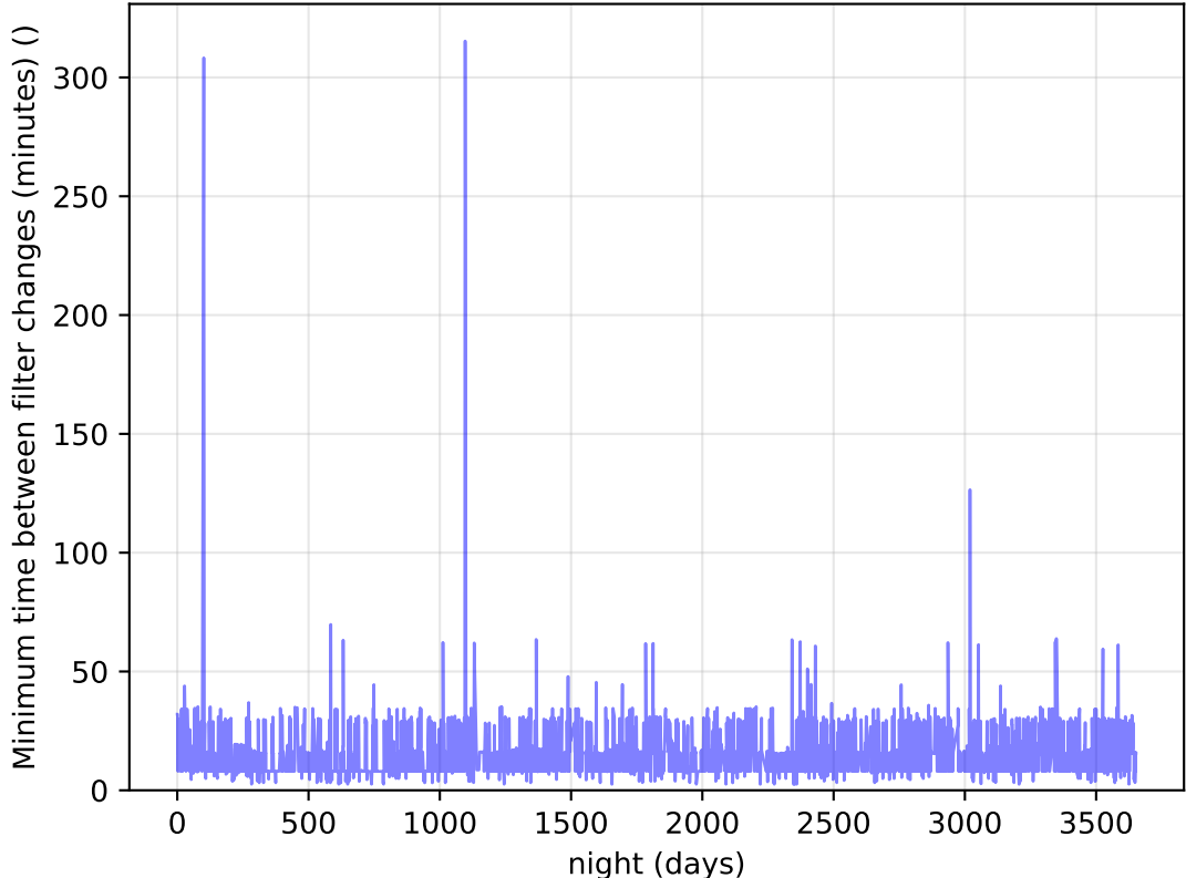
internal_u_expt45_nscale1.0v3.4_10yrs Per Night: Minimum time between filter changes (minutes)
