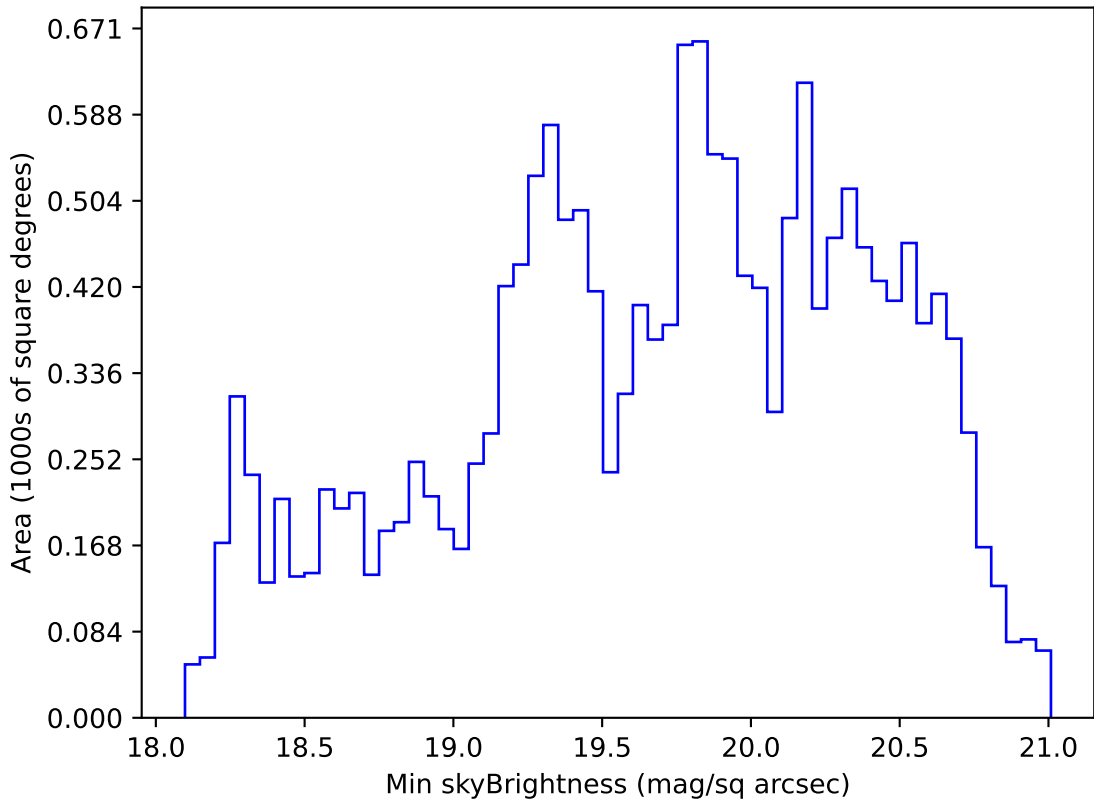
internal_u_expt45_nscale1.0v3.4_10yrs WFD g band: Min skyBrightness
