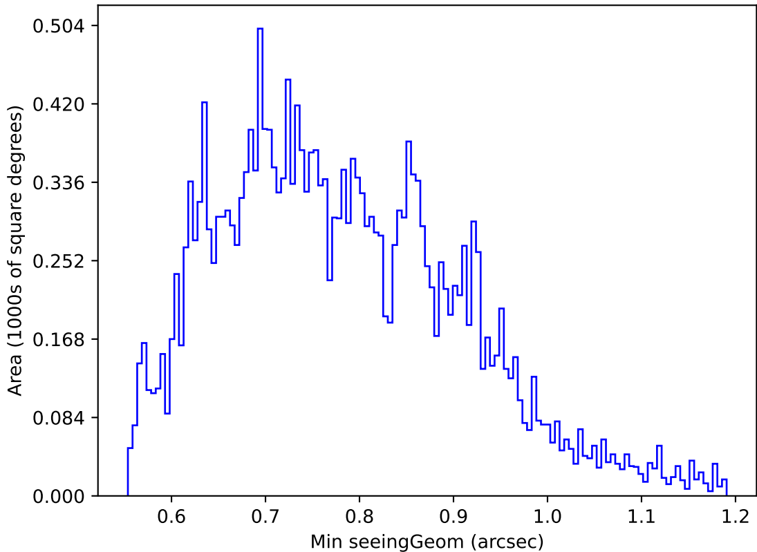
internal_u_expt45_nscale1.0v3.4_10yrs Yr 1 u band: Min seeingGeom
