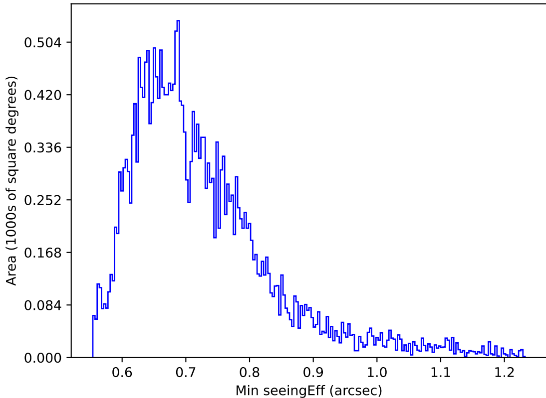
internal_u_expt45_nscale1.0v3.4_10yrs Yr 1 z band: Min seeingEff
