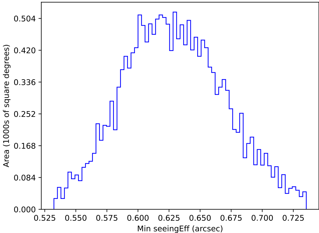
internal_u_expt45_nscale1.0v3.4_10yrs WFD y band: Min seeingEff
