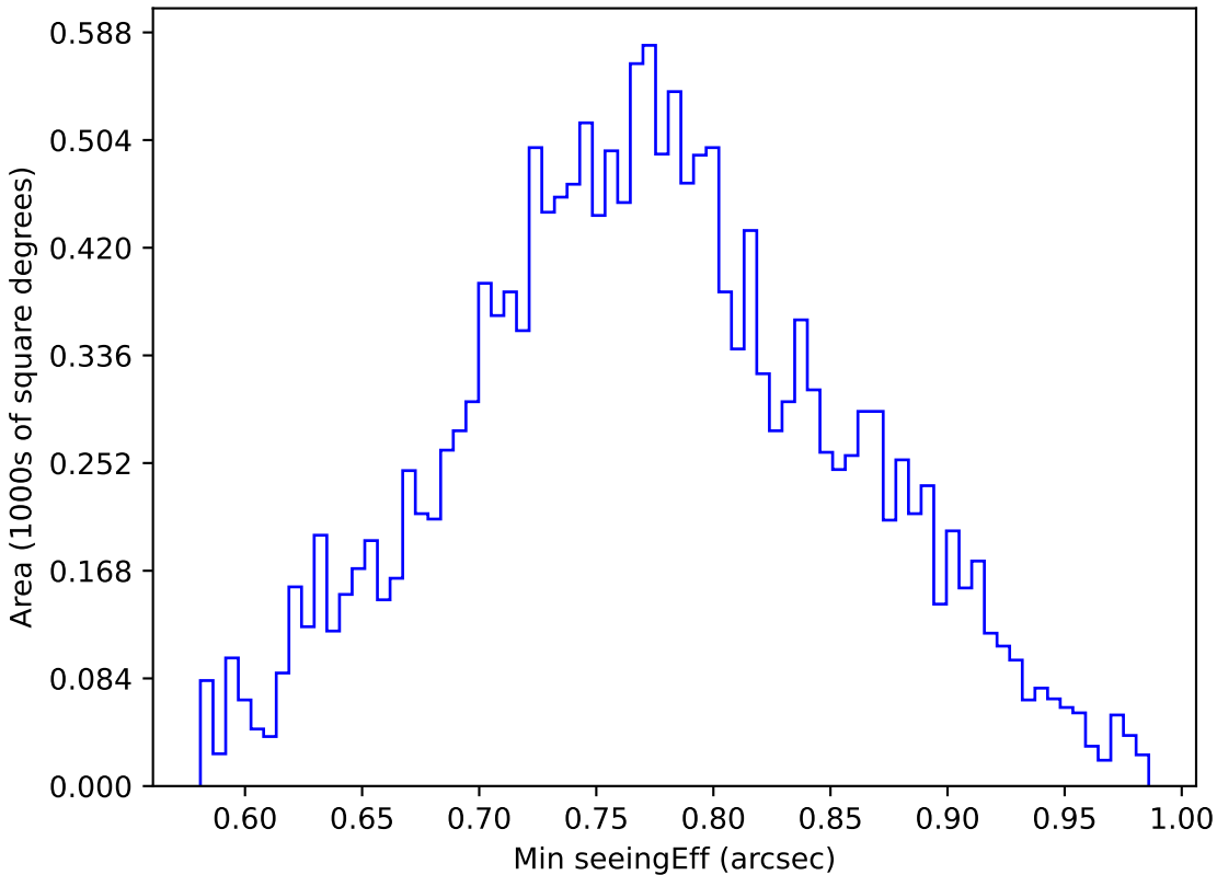
internal_u_expt45_nscale1.0v3.4_10yrs WFD u band: Min seeingEff
