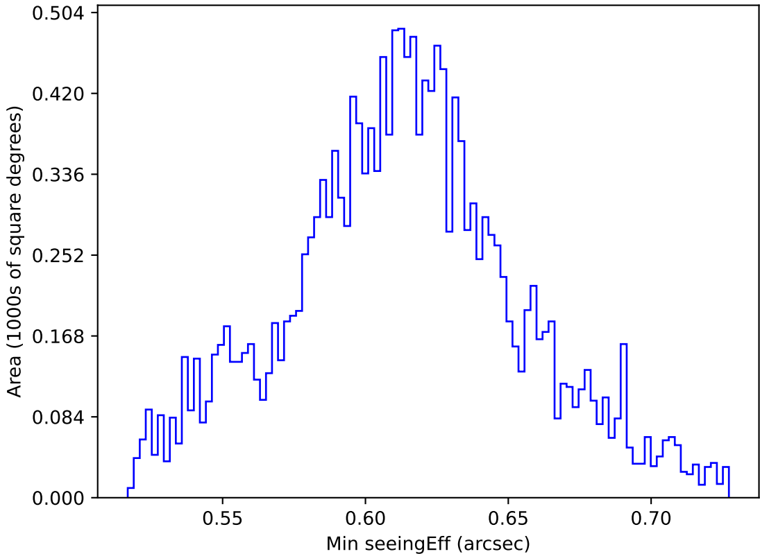
internal_u_expt45_nscale1.0v3.4_10yrs WFD r band: Min seeingEff
