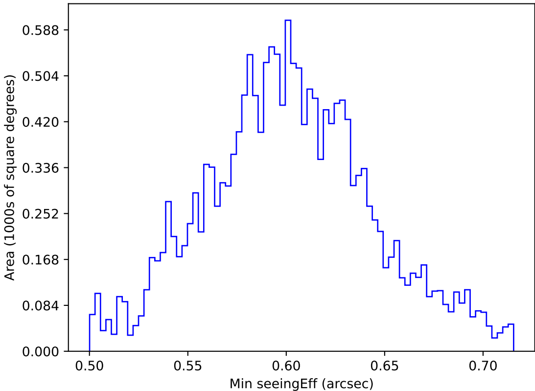
internal_u_expt45_nscale1.0v3.4_10yrs WFD i band: Min seeingEff
