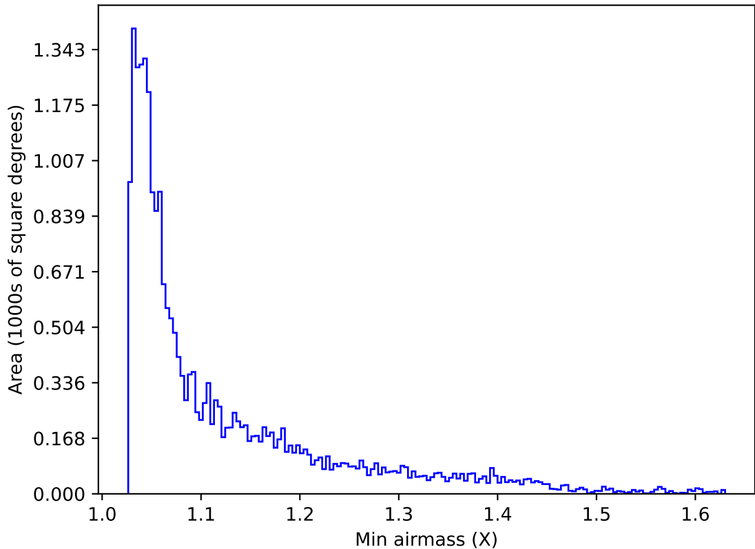
internal_u_expt45_nscale1.0v3.4_10yrs Yr 1 y band: Min airmass
