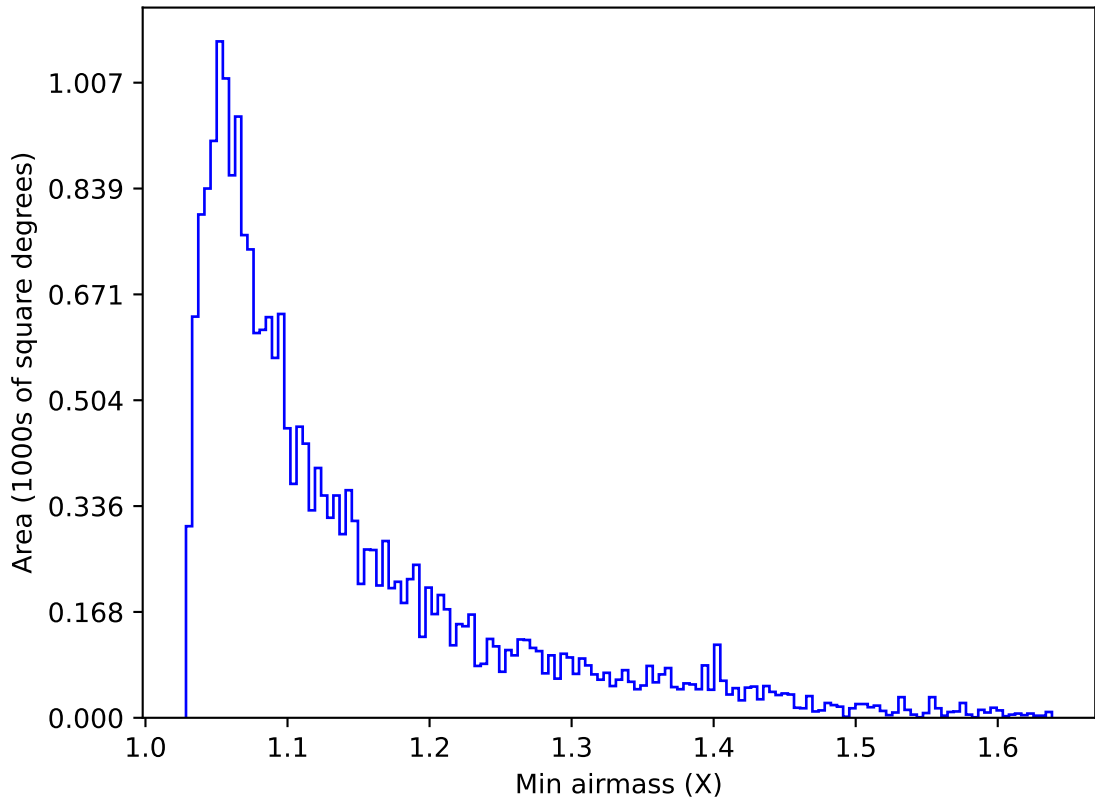
internal_u_expt45_nscale1.0v3.4_10yrs Yr 1 u band: Min airmass
