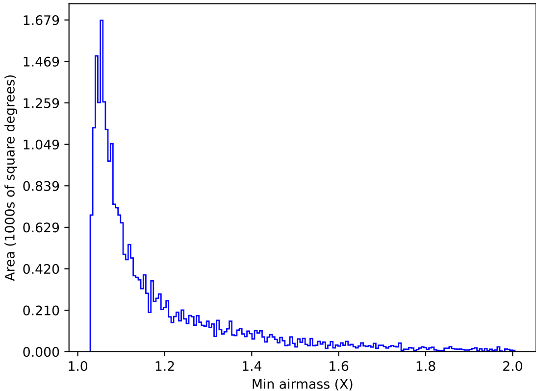
internal_u_expt45_nscale1.0v3.4_10yrs Yr 1 g band: Min airmass
