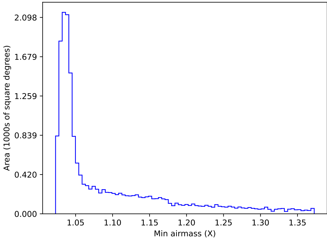
internal_u_expt45_nscale1.0v3.4_10yrs WFD g band: Min airmass
