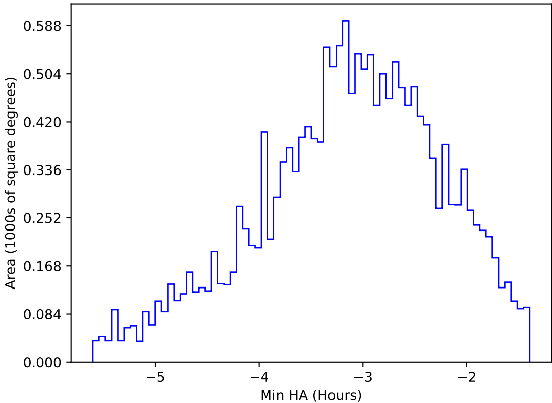
internal_u_expt45_nscale1.0v3.4_10yrs WFD u band: Min HA
