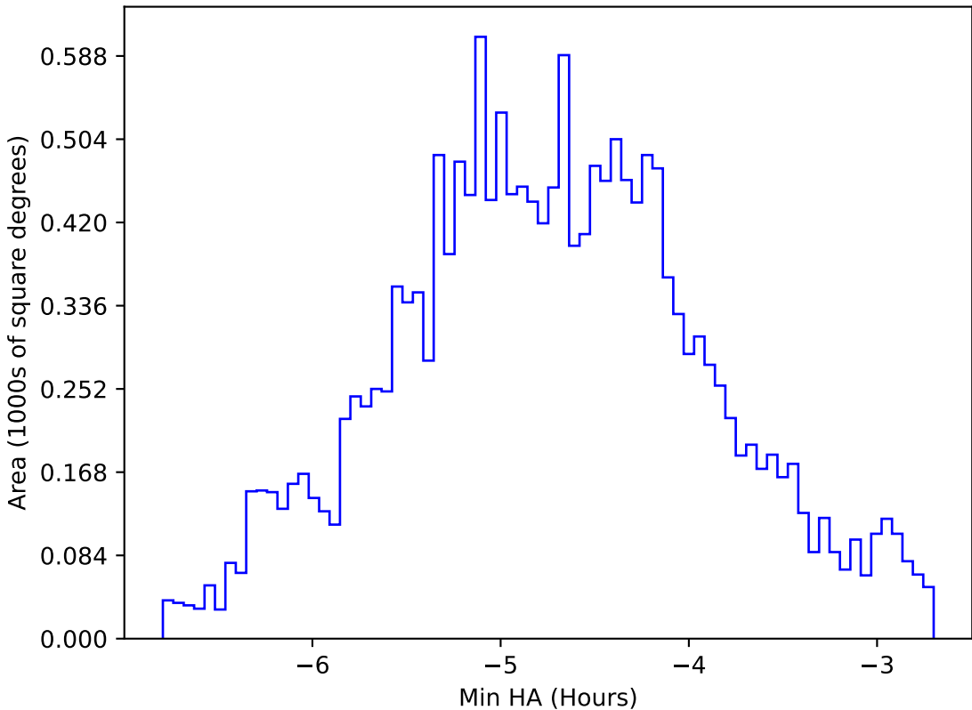
internal_u_expt45_nscale1.0v3.4_10yrs WFD all bands: Min HA
