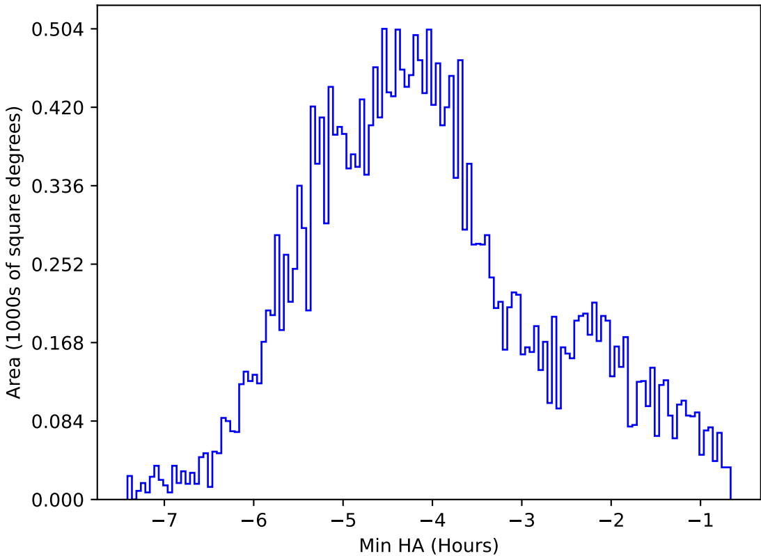
internal_u_expt45_nscale1.0v3.4_10yrs All sky z band: Min HA
