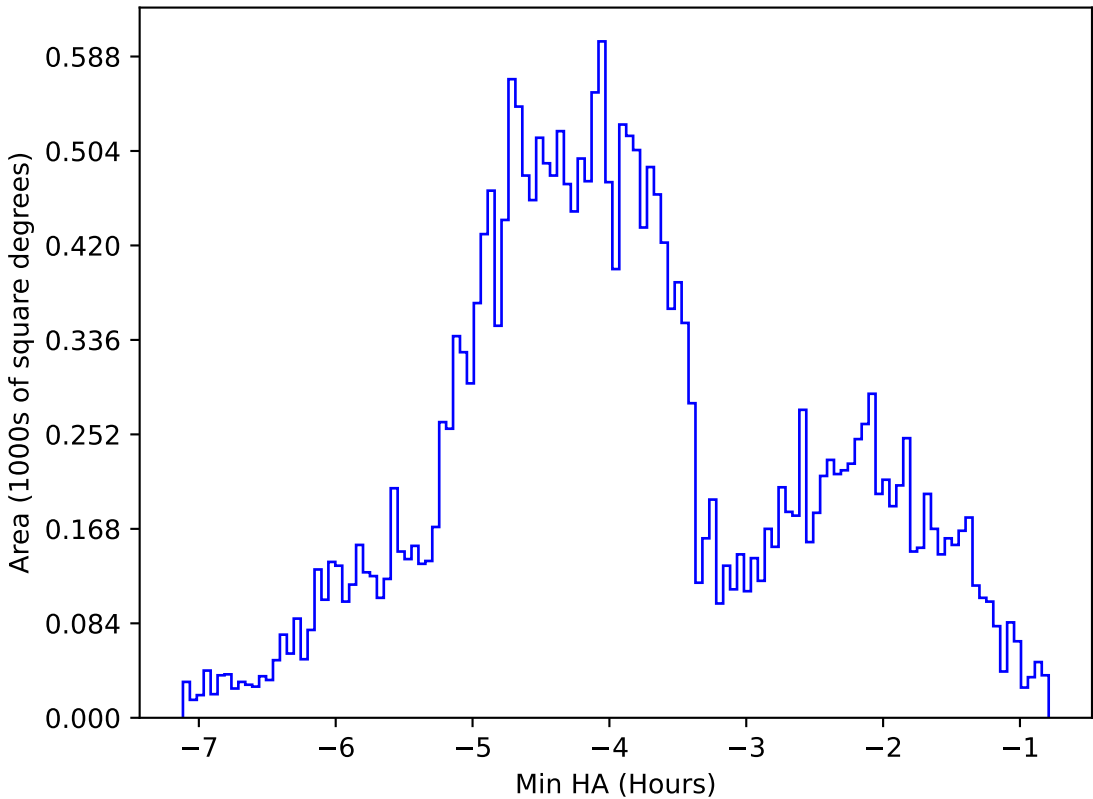
internal_u_expt45_nscale1.0v3.4_10yrs All sky g band: Min HA
