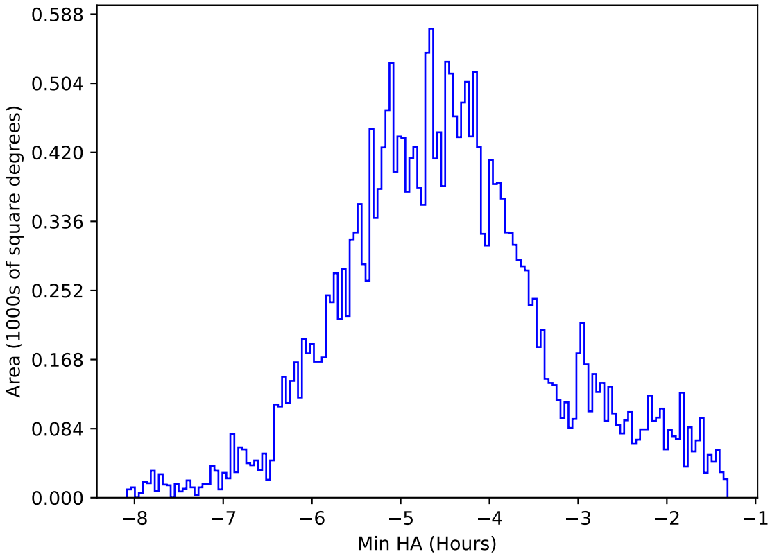
internal_u_expt45_nscale1.0v3.4_10yrs All sky all bands: Min HA
