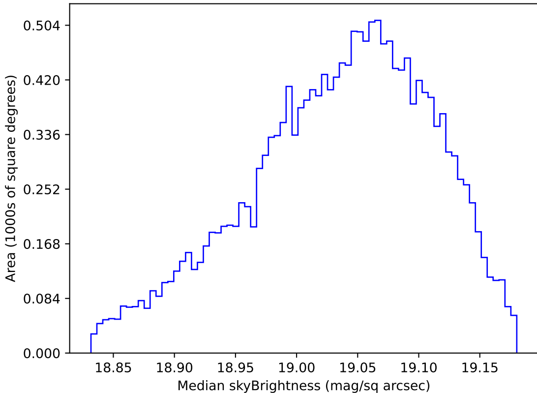
internal_u_expt45_nscale1.0v3.4_10yrs WFD z band: Median skyBrightness
