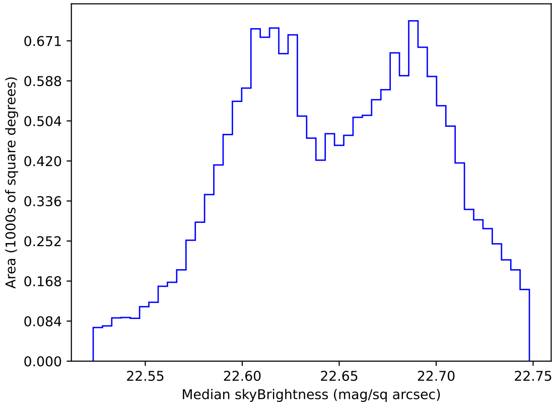
internal_u_expt45_nscale1.0v3.4_10yrs WFD u band: Median skyBrightness
