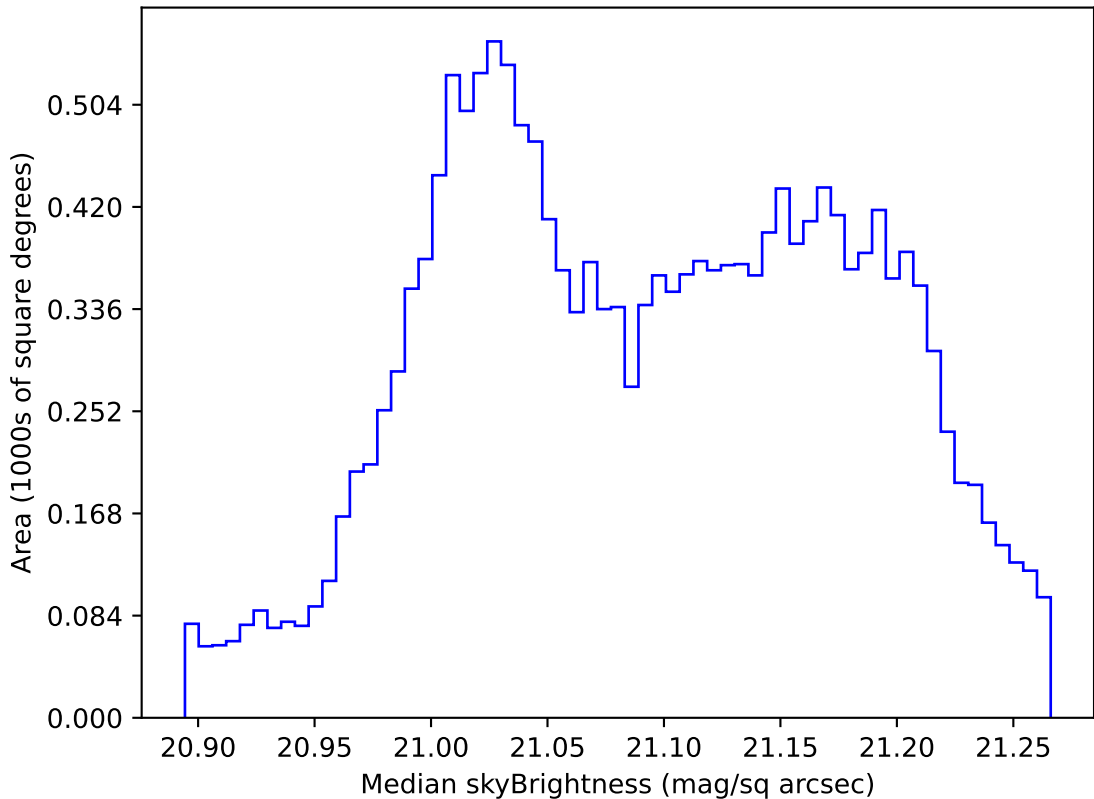
internal_u_expt45_nscale1.0v3.4_10yrs WFD r band: Median skyBrightness
