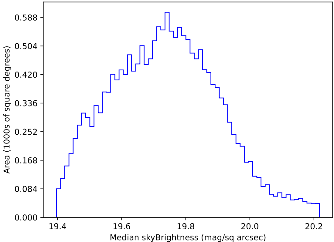
internal_u_expt45_nscale1.0v3.4_10yrs WFD all bands: Median skyBrightness
