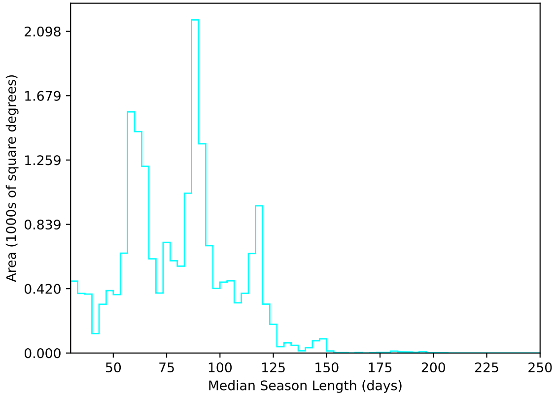
internal_u_expt45_nscale1.0v3.4_10yrs All sky u band: Median Season Length
