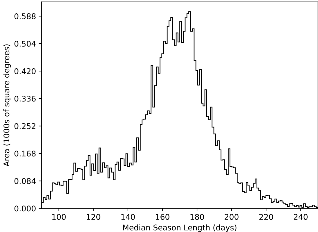
internal_u_expt45_nscale1.0v3.4_10yrs All sky all bands: Median Season Length
