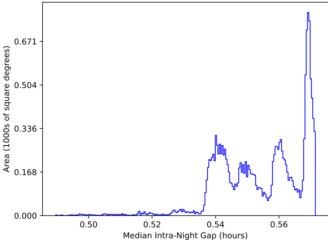
internal_u_expt45_nscale1.0v3.4_10yrs WFD: Median Intra-Night Gap
