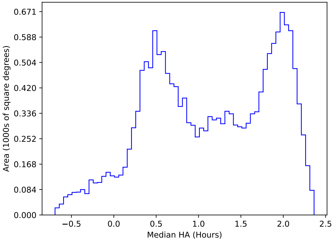
internal_u_expt45_nscale1.0v3.4_10yrs WFD z band: Median HA
