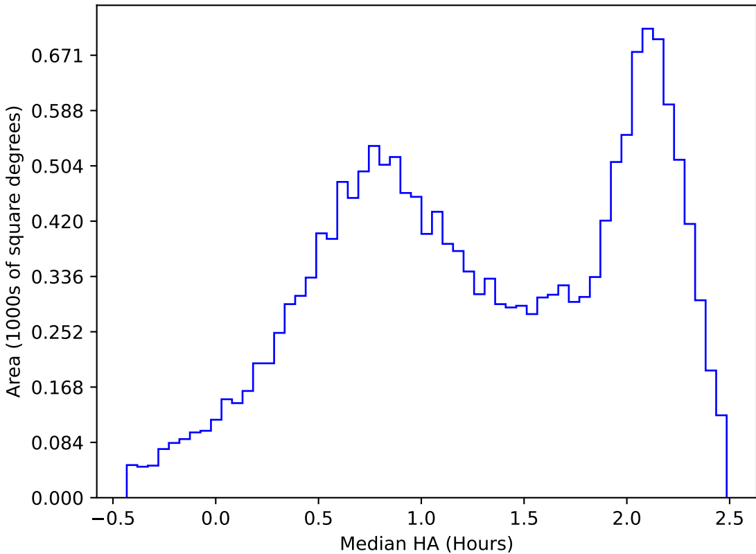
internal_u_expt45_nscale1.0v3.4_10yrs WFD y band: Median HA
