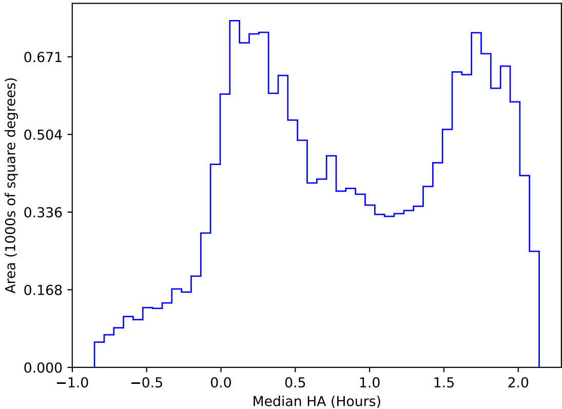
internal_u_expt45_nscale1.0v3.4_10yrs WFD r band: Median HA
