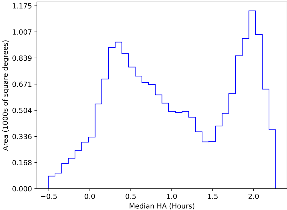
internal_u_expt45_nscale1.0v3.4_10yrs WFD i band: Median HA
