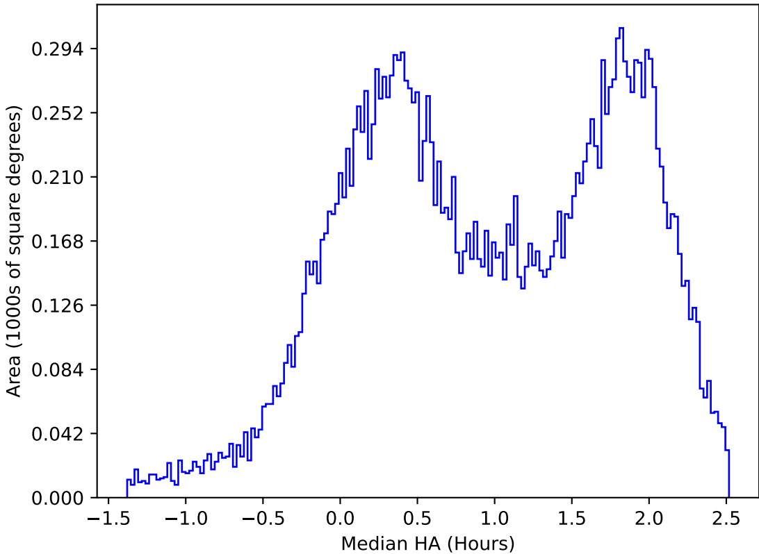
internal_u_expt45_nscale1.0v3.4_10yrs All sky u band: Median HA
