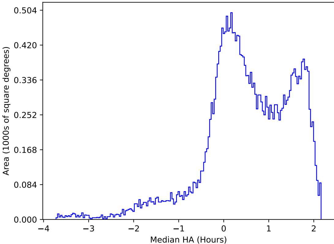
internal_u_expt45_nscale1.0v3.4_10yrs All sky g band: Median HA
